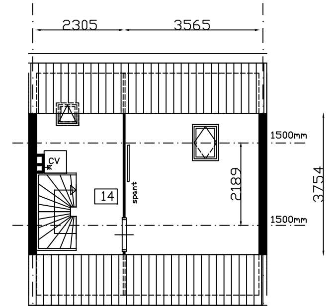
ZOLDER
